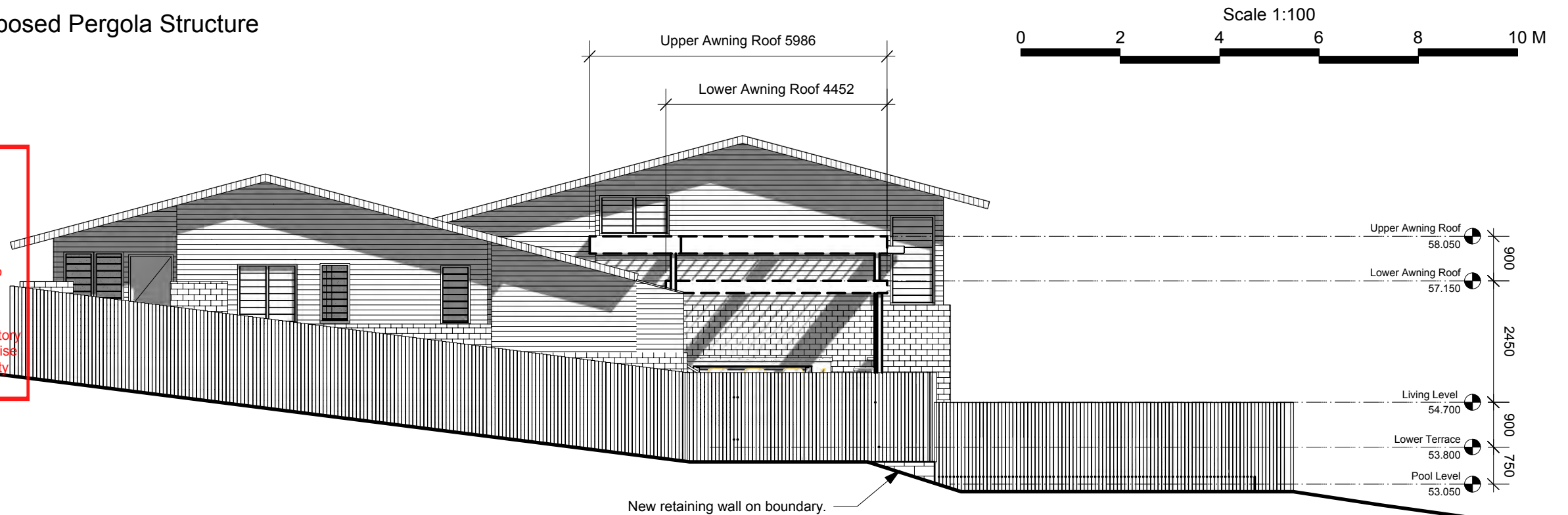
East Elevation - Proposed Pergola Structure Scale 1:100
